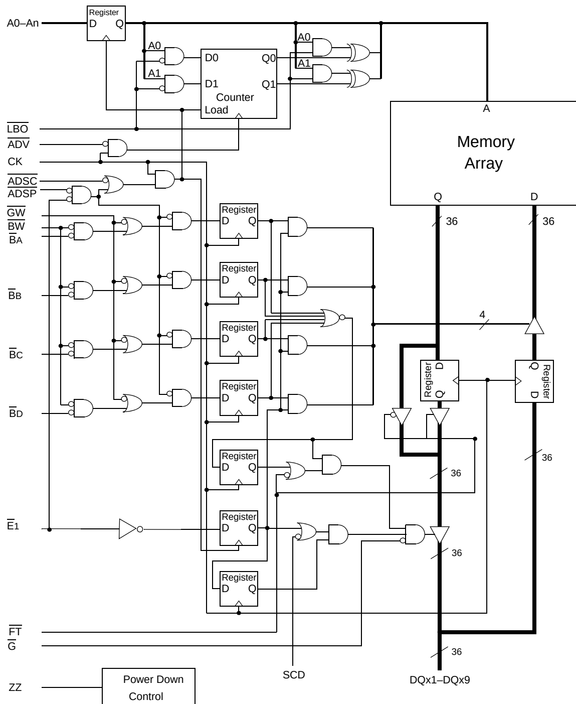
GS816218/36D-xxxV Block Diagram
