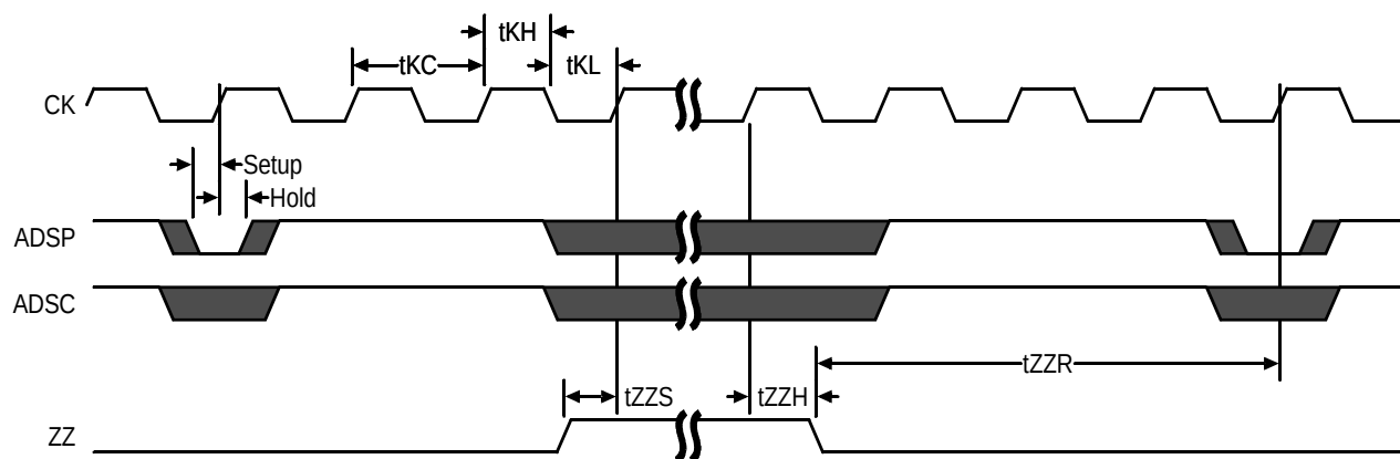
Sleep Mode Timing
