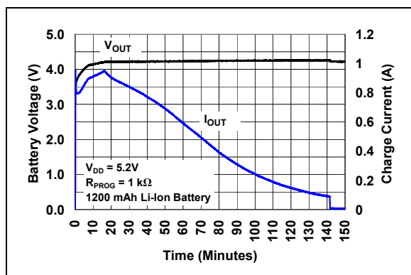
FIGURE 2-26: Complete Charge Cycle (1200 mAh Li-Ion Battery).
