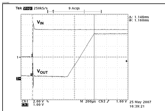
FIGURE 2-25: V_{USB} Start Delay (USB = High)
