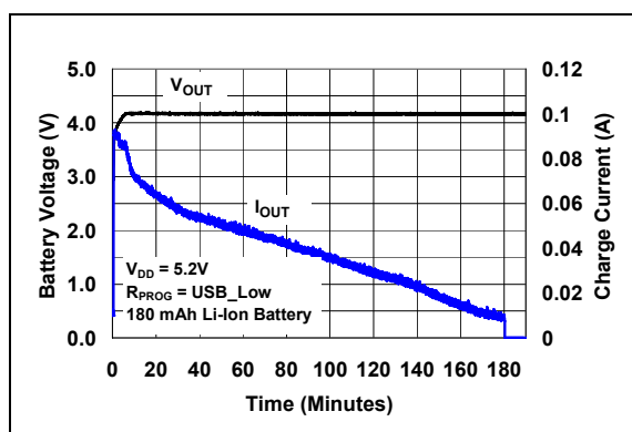
FIGURE 2-28: Complete Charge Cycle (180 mAh Li-Ion Battery).
