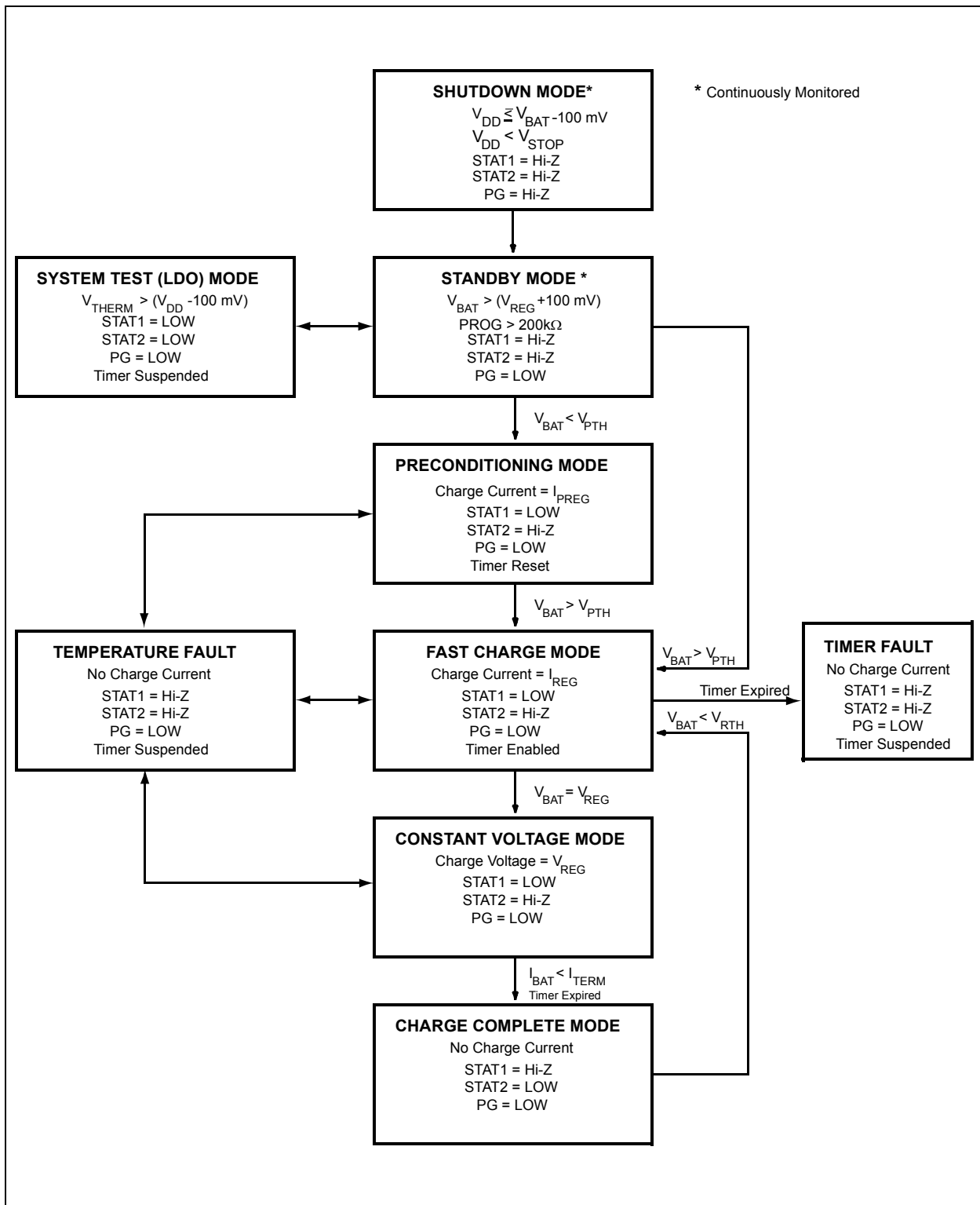
FIGURE 4-1: Flow Chart.
