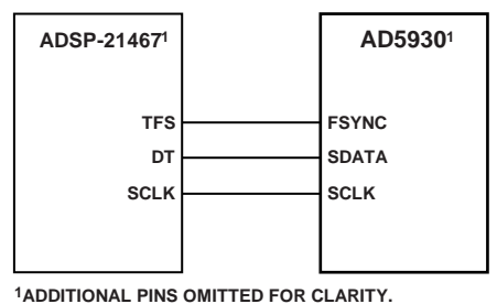
Figure 36. ADSP-21467 to AD5930 Interface
