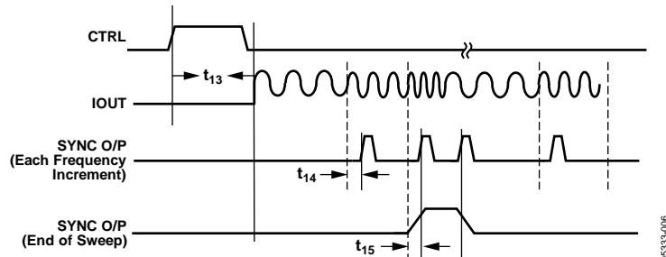
Figure 6. CTRL Timing, Saw-Sweep Mode
