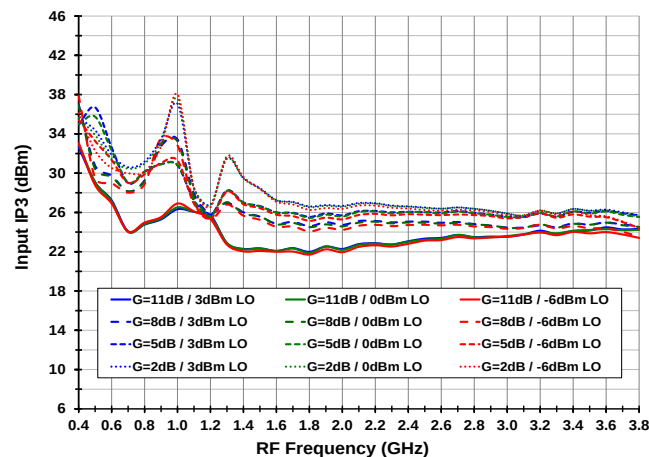
Figure 7. OIP3 vs. LO Power and Gain Setting (Vcc = 3.15, Tcase = 105C)
