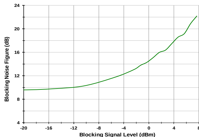
Figure 19. Blocking Noise Figure (Max Gain, LO=1700MHz, RF=1899MHz, Blocker=1999MHz, 25C ambient)
