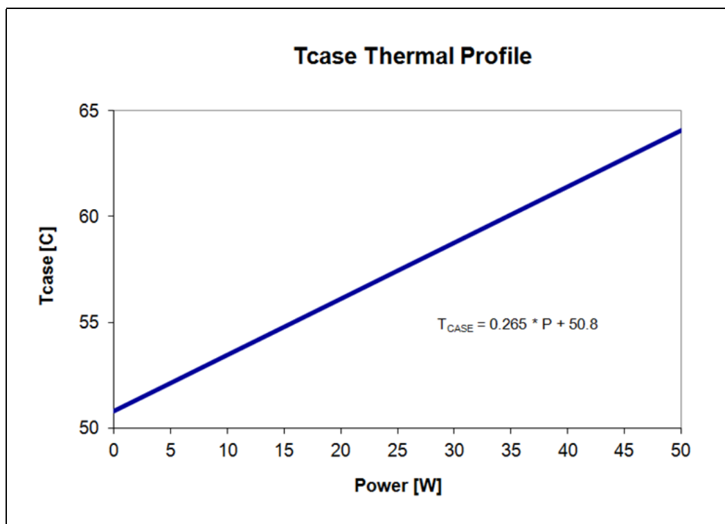
Figure 5-12. Server SKU Platform (8-Core 50W) T CASE Thermal Profile.
