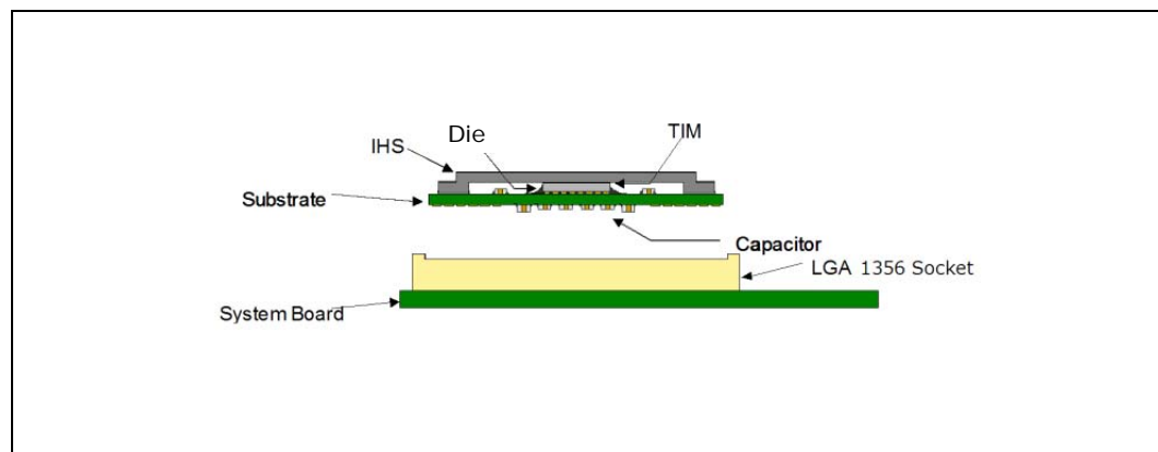
Figure 9-1. Processor Package Assembly Sketch
