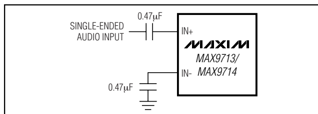
Figure 5. Single-Ended Input
