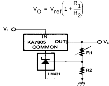
Figure 13. Output Control for Three-Terminals Fixed Regulator
