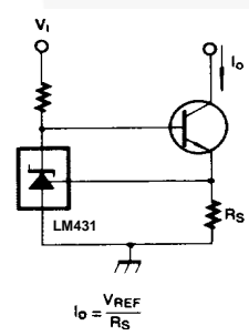
Figure 16. Constant-Current Sink
