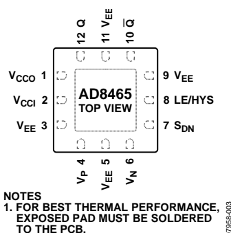
Figure 3. Pin Configuration
