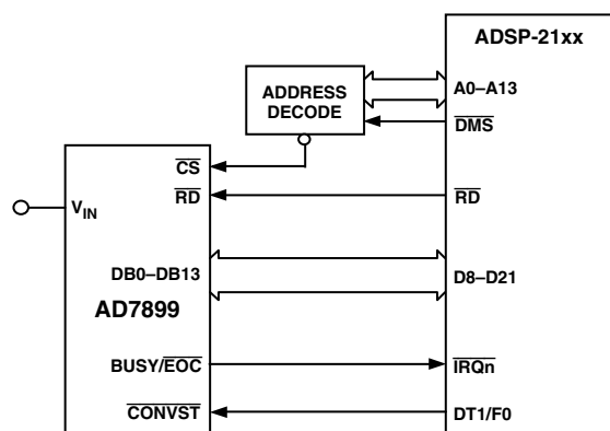
Figure 14. AD7899-ADSP-21xx Interface
