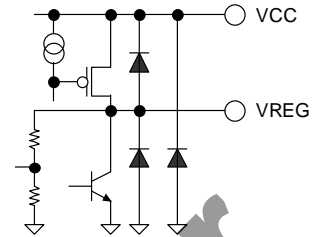
Figure 37. VREG, VCC
