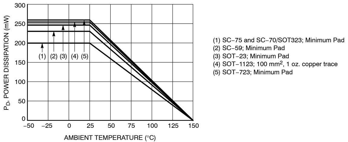
Figure 1. Derating Curve
