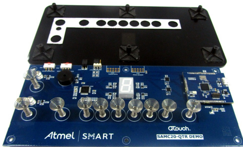
Figure 1-1 Internal View of the Demo Kit
