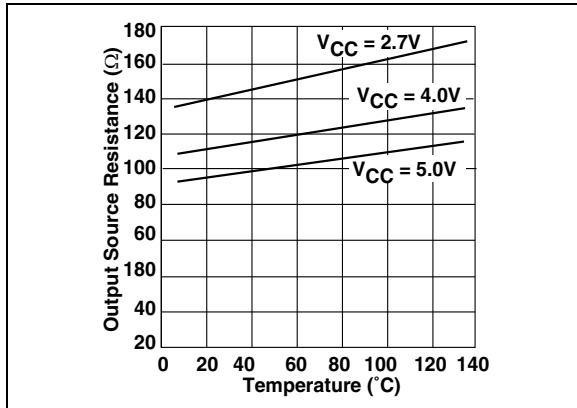
FIGURE 2-7: Output Source Resistance vs. Temperature (TC6502).
