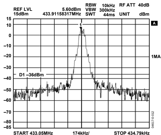
Figure 11. Phase Noise Response— I_{CP} = 2.0 \text{ mA} , I_{VC0} = 2.0 \text{ mA} , RF_{OUT} = 433.92 \text{ MHz} , PFD = 4 \text{ MHz} , PA \text{ Bias} = 5.5 \text{ mA}
