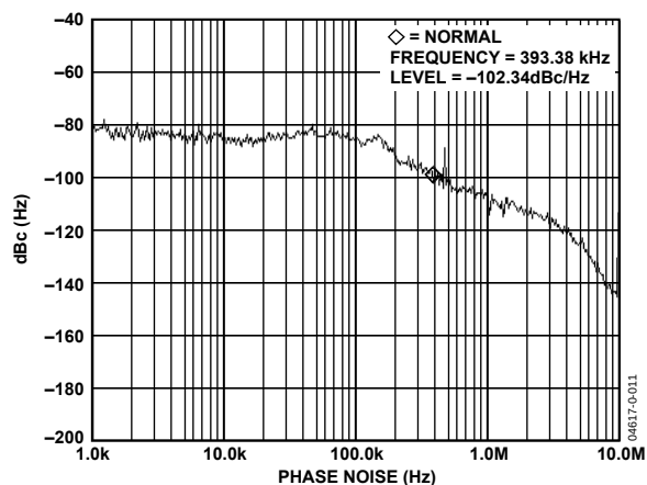
Figure 11. Phase Noise Response— I_{CP} = 2.0 \text{ mA} , I_{VC0} = 2.0 \text{ mA} , RF_{OUT} = 433.92 \text{ MHz} , PFD = 4 \text{ MHz} , PA \text{ Bias} = 5.5 \text{ mA}
