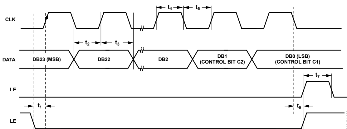
Figure 2. Timing Diagram
