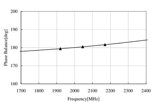
Phase Balance
