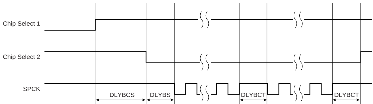
Figure 33-10. Programmable Delays
