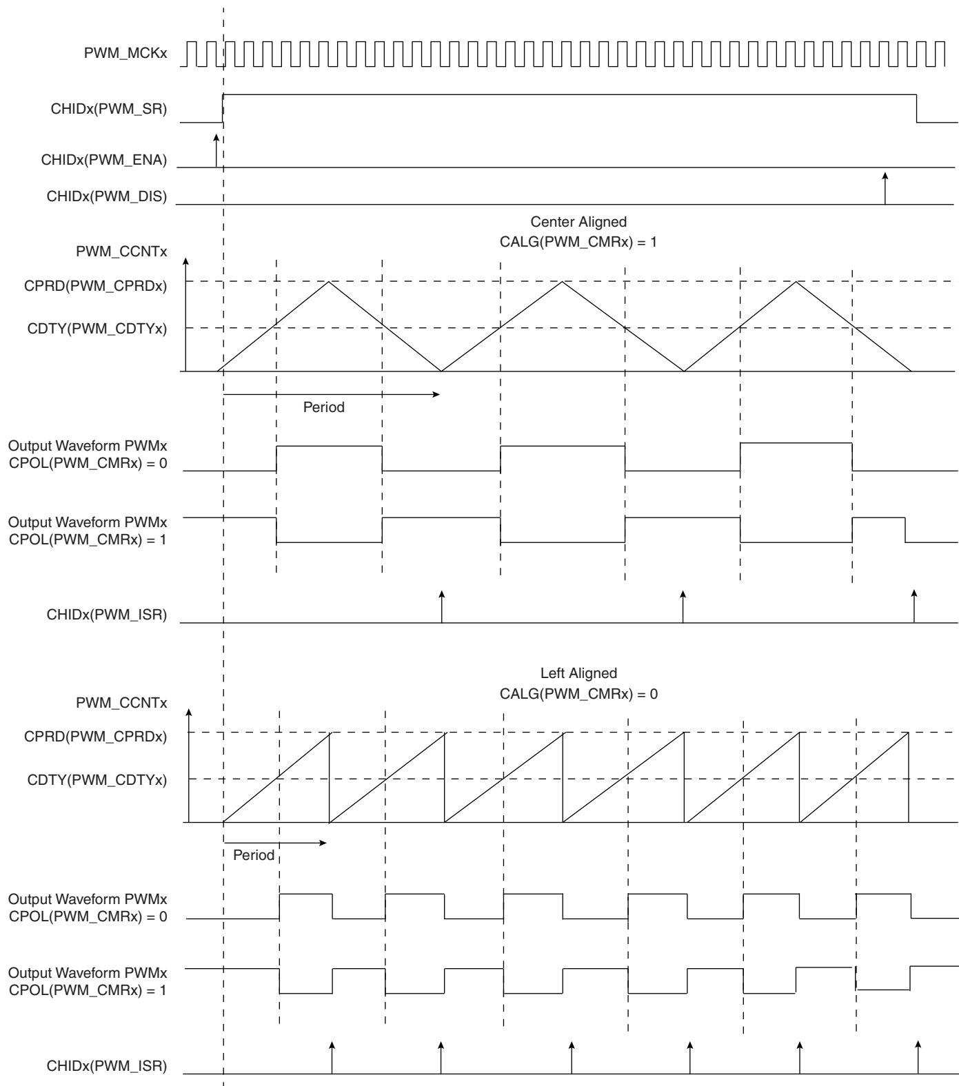
Figure 38-5. Waveform Properties
