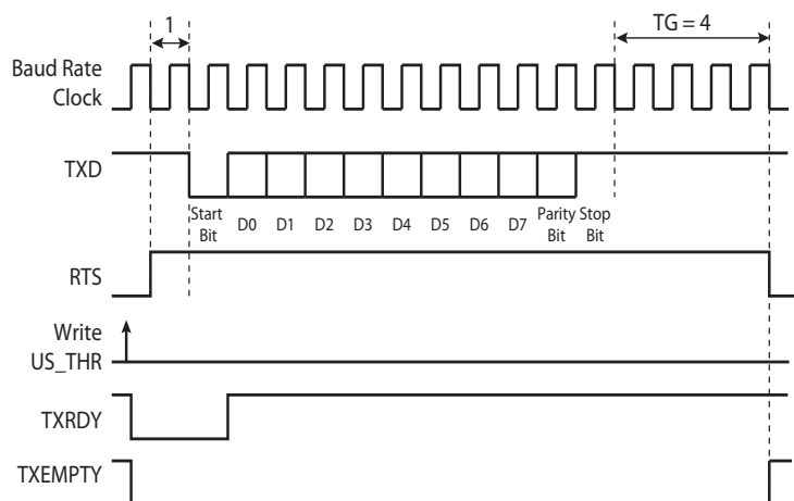
Figure 36-36. Example of RTS Drive with Timeguard
