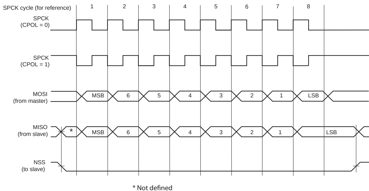
Figure 33-4. SPI Transfer Format (NCPHA = 0, 8 bits per transfer)
