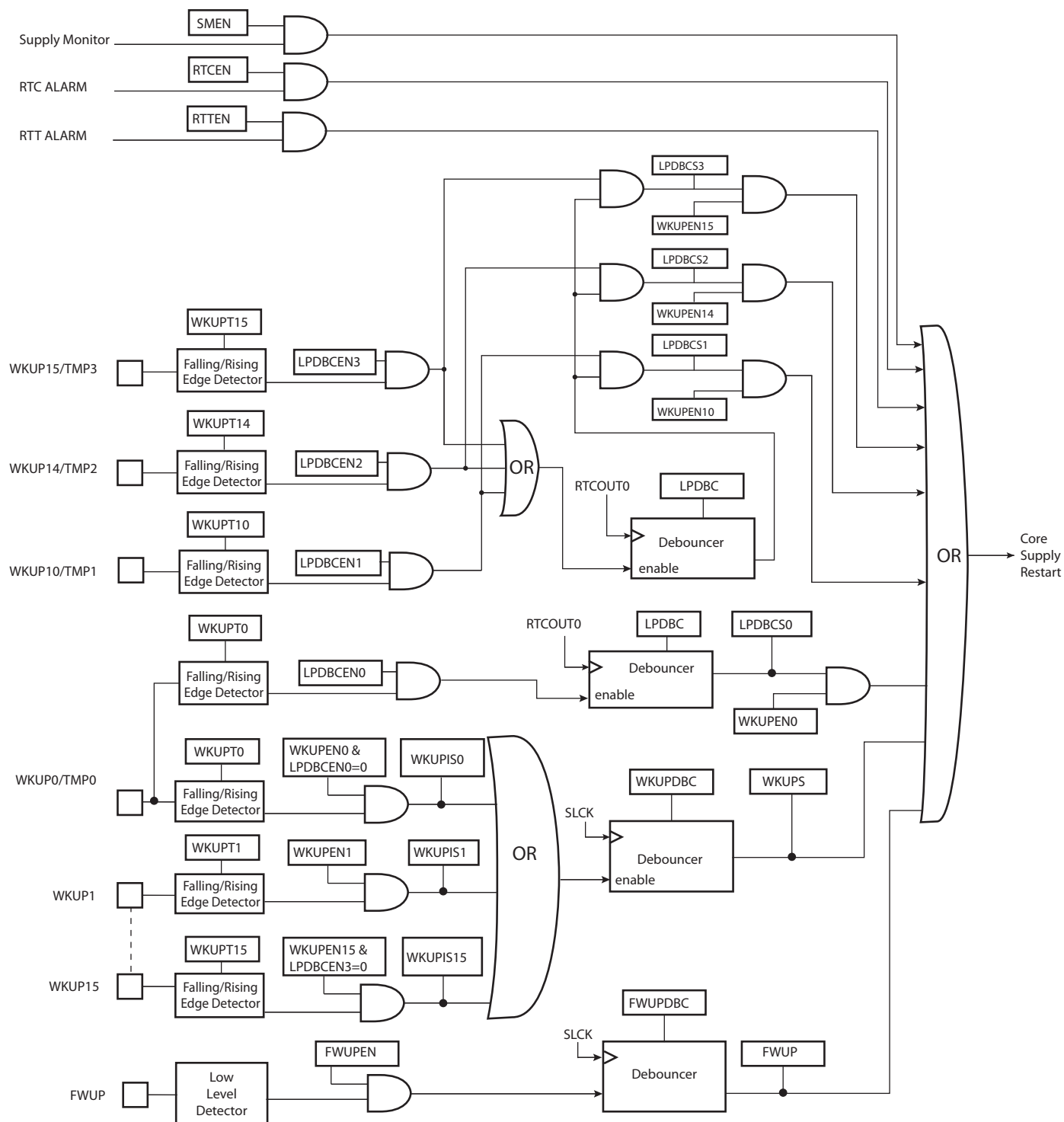
Figure 20-4. Wake-up Sources
