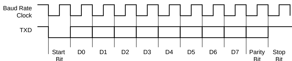
Figure 36-5. Character Transmit
