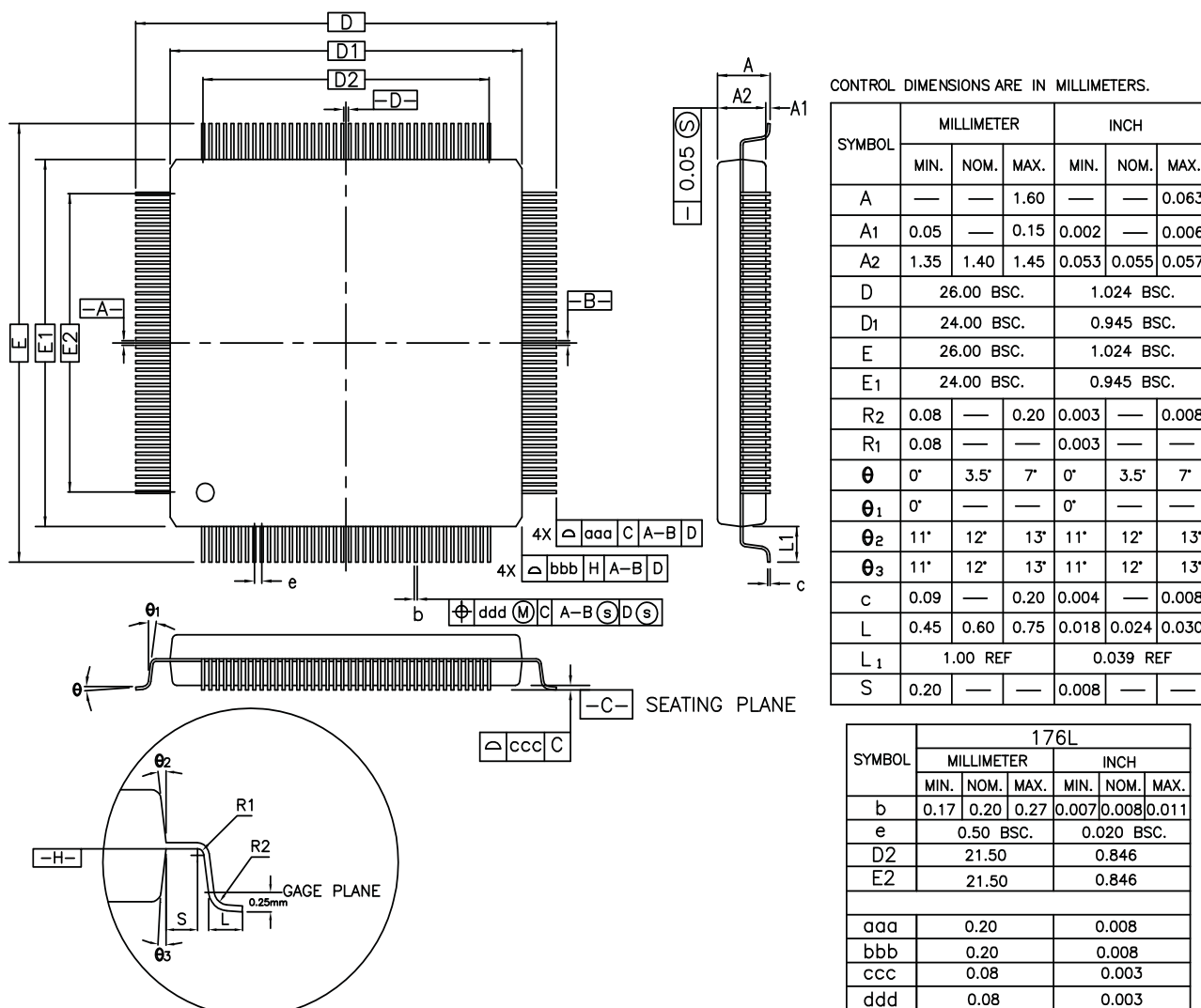
Figure 46-1. 176-lead LQFP Package Drawing
