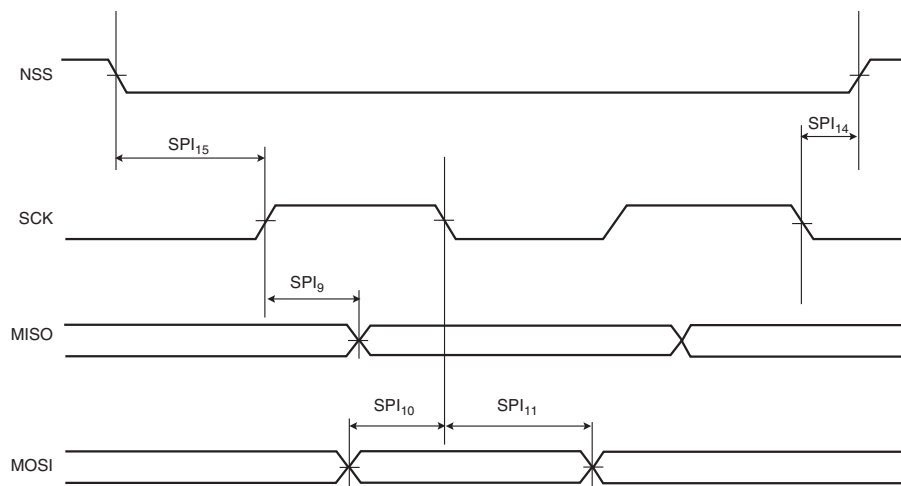
Figure 45-7. USART SPI Slave Mode: (Mode 0 or 3)
