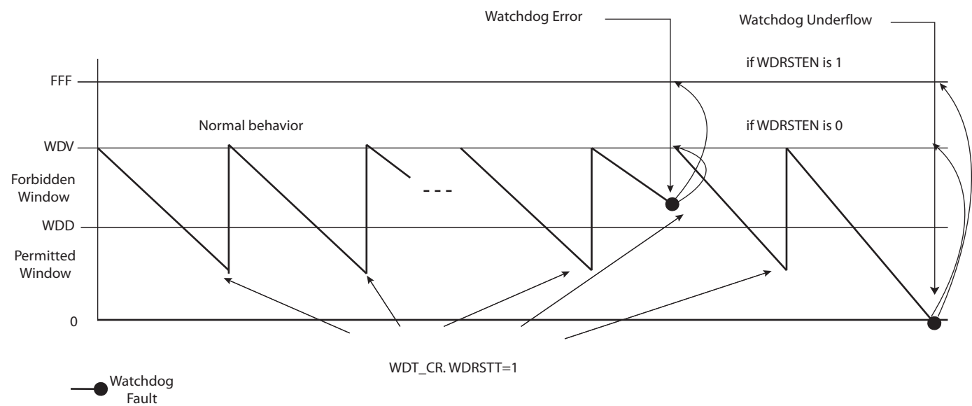
Figure 18-2. Watchdog Behavior
