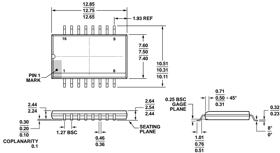
COMPLIANT TO JEDEC STANDARDS MS-013-AC Figure 40. 16-Lead Standard Small Outline Package, with Increased Creepage [SOIC_IC] Wide Body (RI-16-2) Dimensions shown in millimeters
