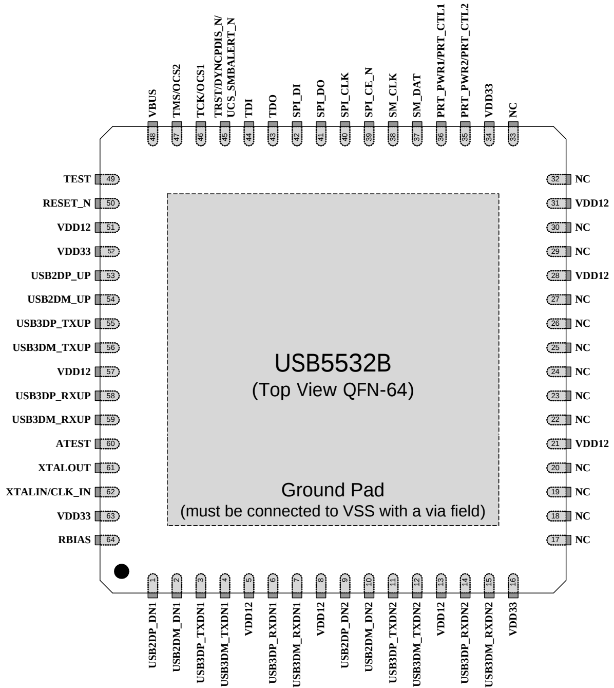
FIGURE 3-1: USB5532B 64-PIN QFN
