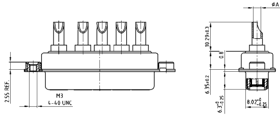
Mounting style: Threaded insert
