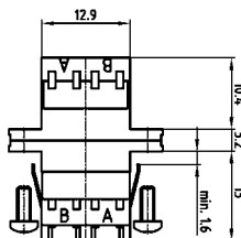
Adapter with flange
