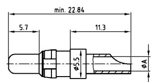
Plug contact
