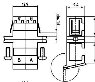
Adapter with shutter
