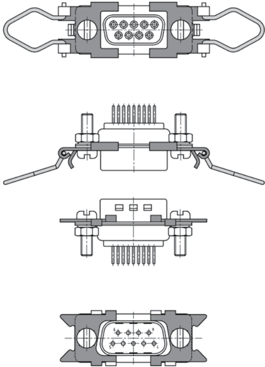
View for assembly
