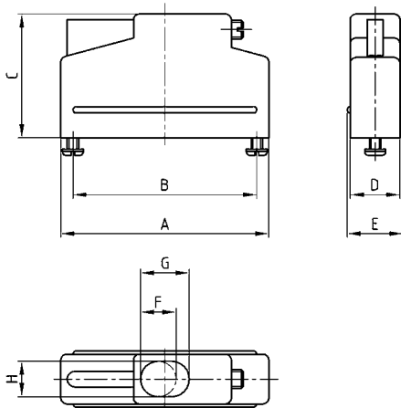
Straight cable entry
