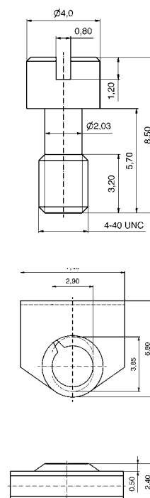
Type 3: Brass
