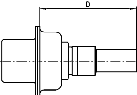
Installation dimension
