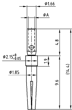
Signal socket crimp contact (Standard version)
