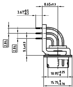
Shell size 5
