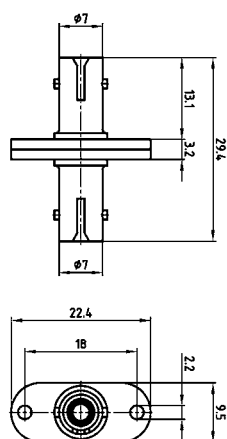
Simplex-Adapter
