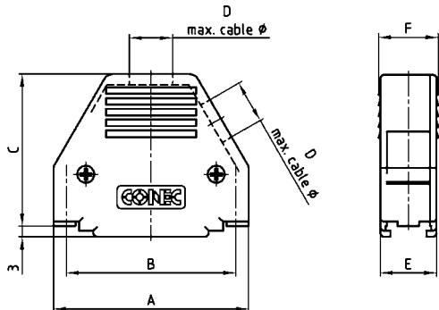
Housing with slide lock
