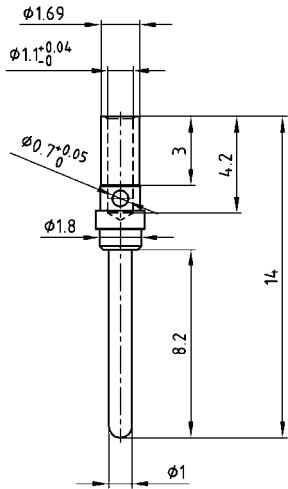
Signal plug crimp contact (Standard version)
