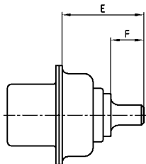
Installation dimension
