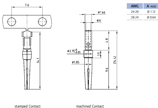
stamped Contact
