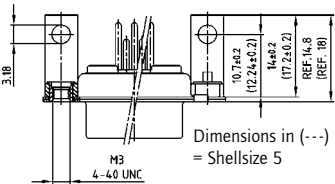
Shell size 5
