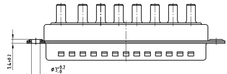
Mounting style: Through-hole
