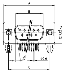
PCB-Layout: Kat1kGHA
