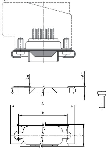
Type 3
