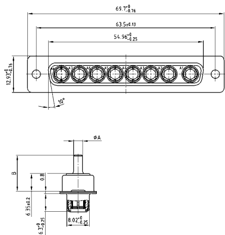
Mounting style: Through-hole
