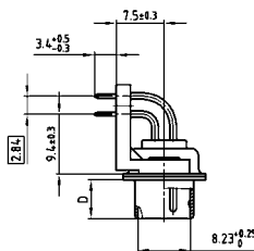
Shell size 1-4
