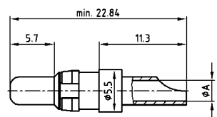
Plug contact
