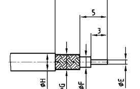
Wire stripping
