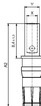
Power crimp contact (short version)
