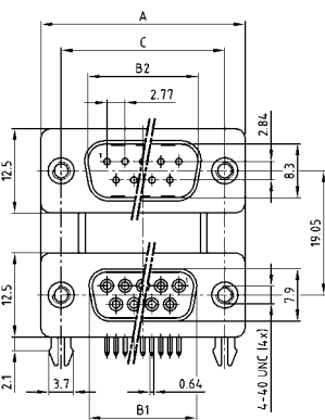
Connector spacing 19.05 mm
