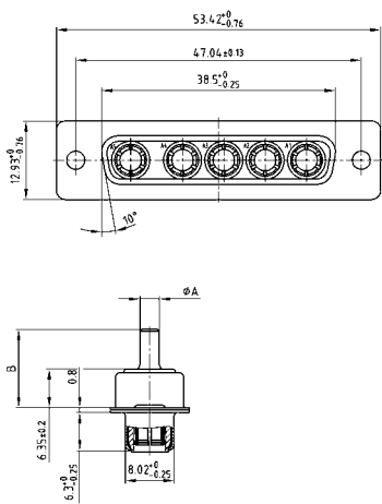
Mounting style: Through-hole
