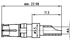
Socket contact
