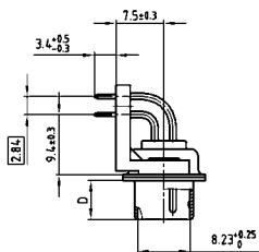
Shell size 1-4
