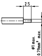
Wire stripping
