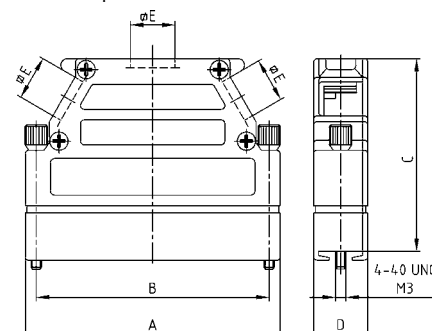
Cable clamp
