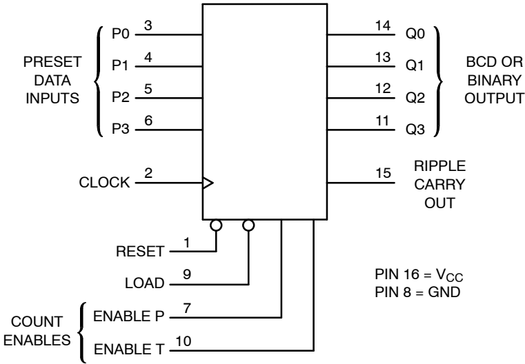
Figure 2. Logic Diagram
