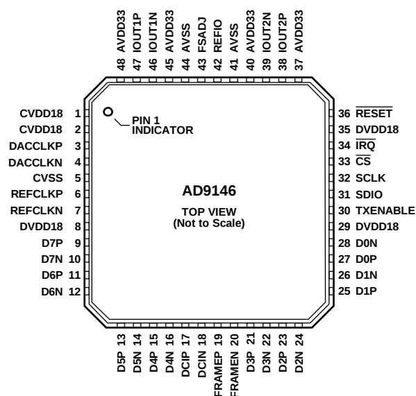
Figure 3. Pin Configuration
