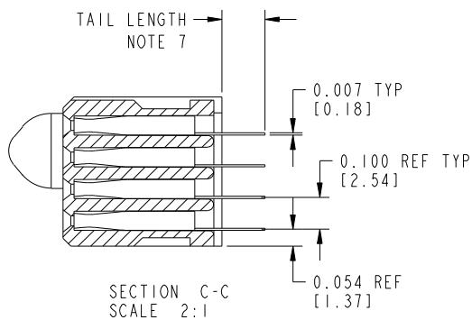
mat'l code SEE NOTE 2 tolerances unless otherwise specified CUSTOMER www.fciconnect.com litr ecn no. dr date linear .XX±.01 / .X±0.3 COPY title VERTICAL RECEPTACLE w/GUIDE PIN POWER / SIGNAL / POWER R .XXX±.005 / .XX±0.13 projection angles ° ± ° dr D. EATON 05-25-99 product family PwrBlade code 213 engr RYAN YUAN 11/08/06 size dwg no sheet chr J. BROWN 05-24-99 of appd J. BROWN 05-24-99 scale A 51740 3 of sheet index revision sheet
