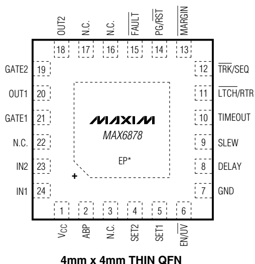
4mm x 4mm THIN QFN
