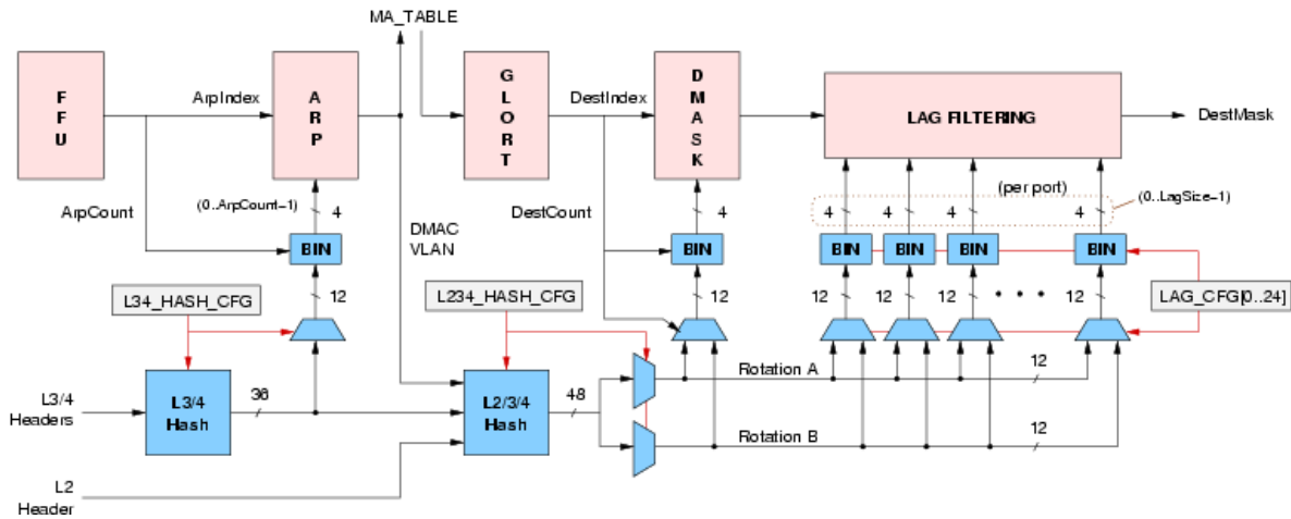
Figure 10-1 Frame Hashing
