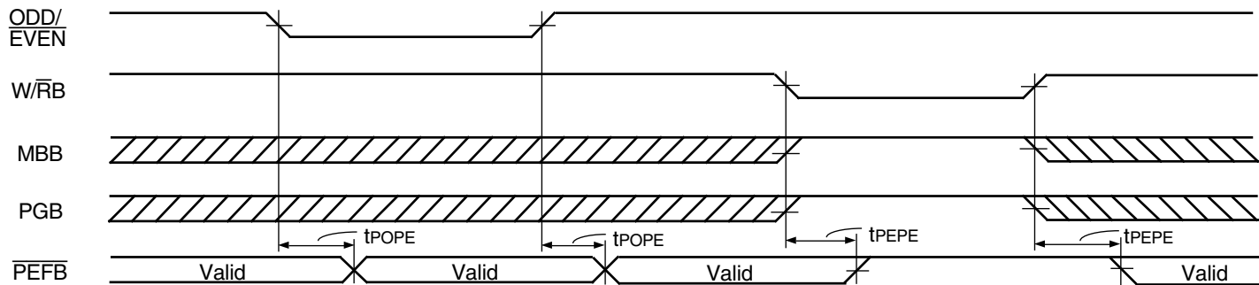
Figure 18. ODD/ \overline{\text{EVEN}} \overline{\text{W/RB}} , MBB, and PGB to \overline{\text{PEFB}} Timing
