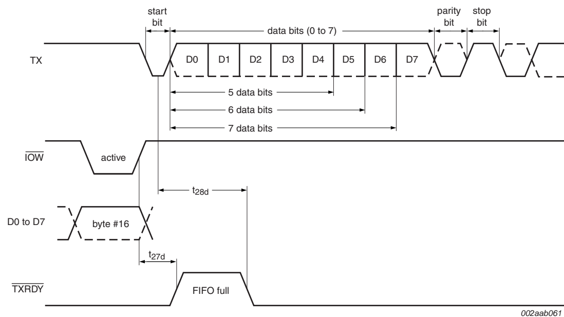
Fig 29. Transmit ready timing in FIFO mode (DMA mode '1')
