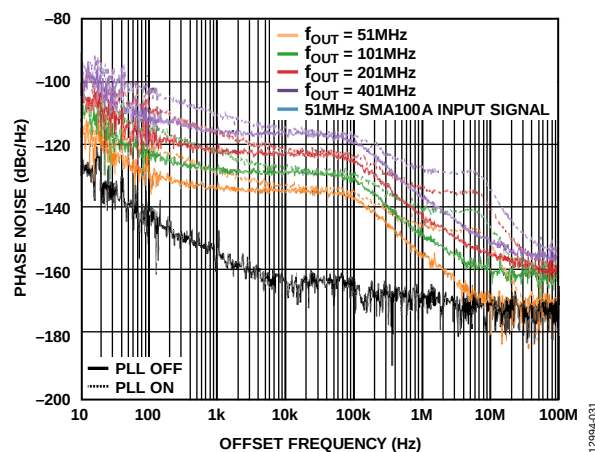
Figure 31. Single Tone Phase Noise vs. Offset Frequency at Four f_{OUT} Values and with an SMA100A Signal Generator, f_{DAC} = 1.96608 GHz, PLL On and Off
