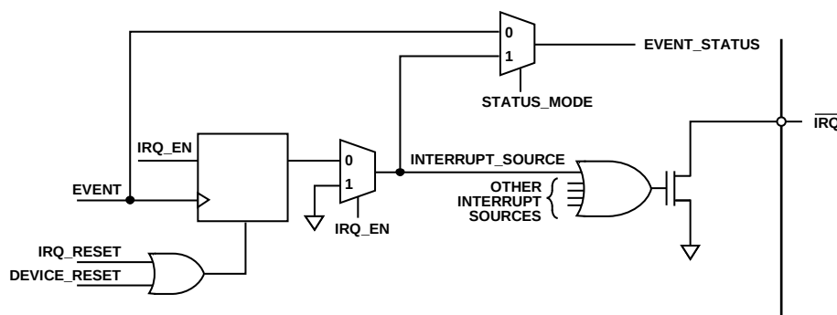
Figure 68. Simplified Schematic of \overline{IRQ} Circuitry
