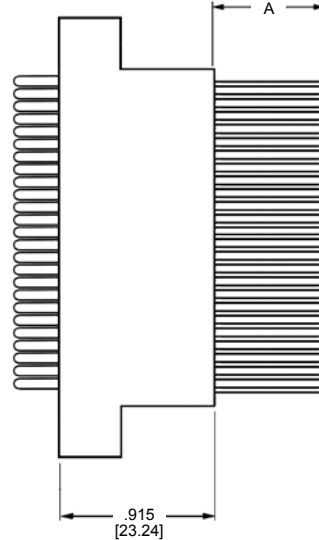
Plug Assembly
