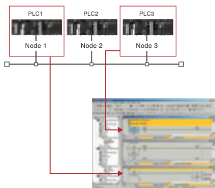
CX-Programmer
