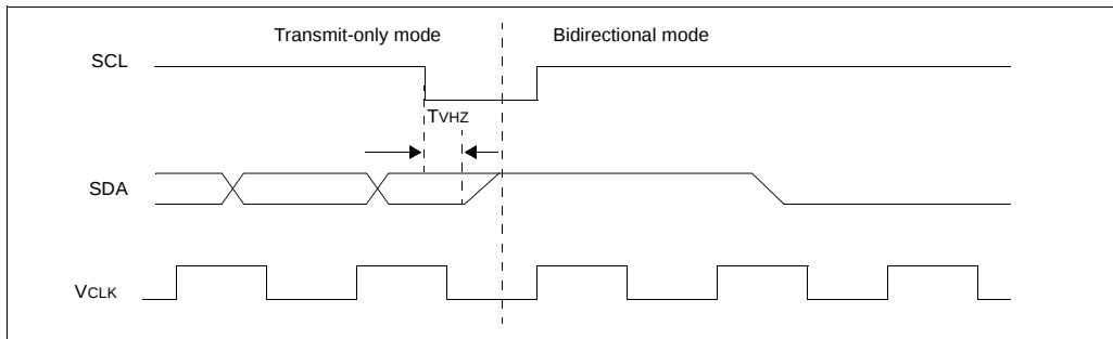
FIGURE 3-1: MODE TRANSITION
