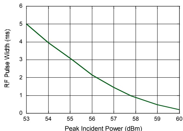
Pulse Width vs. Peak Input Power @ +85^\circ\text{C} (10% Duty Cycle, 1.3 GHz)
