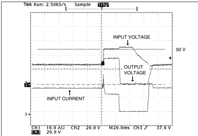
Figure 3 — Transient Immunity: M-FIAM5B output response to an input transient.
