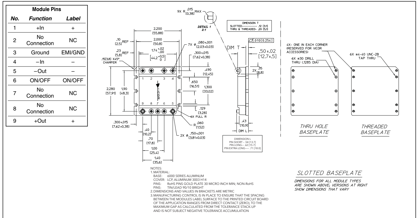
Figure 7 — Mechanical diagram
