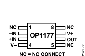
Figure 1. 8-Lead MSOP (RM Suffix)
