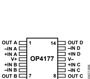
Figure 6. 14-Lead TSSOP (RU Suffix)
