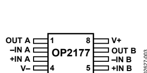
Figure 3. 8-Lead MSOP (RM Suffix)
