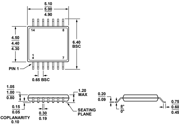
COMPLIANT TO JEDEC STANDARDS MO-153-AB-1 Figure 72. 14-Lead Thin Shrink Small Outline Package [TSSOP] (RU-14) Dimensions shown in millimeters
