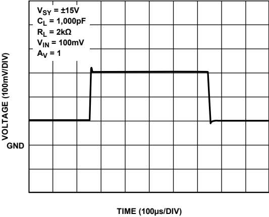
Figure 16. Small Signal Transient Response
