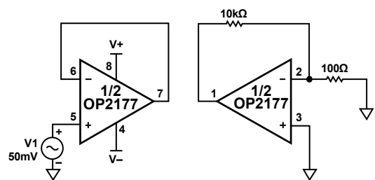
Figure 68. Channel Separation Test Circuit
