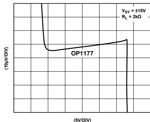
Figure 51. Gain Linearity
