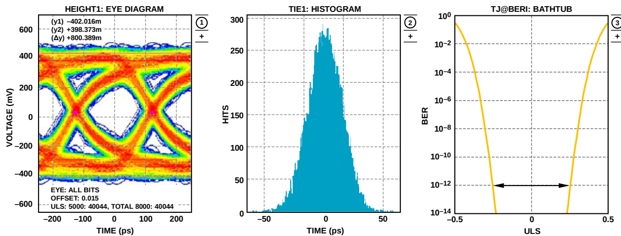
Figure 60. Digital Outputs Data Eye with Trace Lengths Greater Than 12 Inches on Standard FR-4, External 100 \Omega Terminations at Receiver
