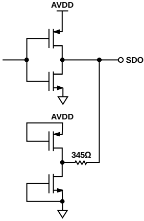
Figure 35. Equivalent SDO Output Circuit
