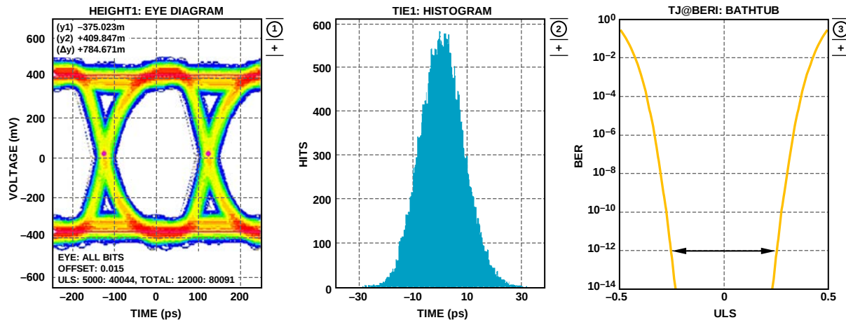
Figure 59. Digital Outputs Data Eye with Trace Lengths Less Than 6 Inches on Standard FR-4, External 100 \Omega Terminations at Receiver
