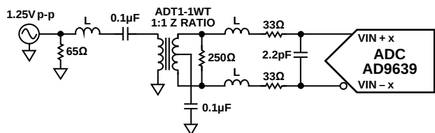
Figure 39. Differential Transformer-Coupled Configuration for Wideband IF Applications
