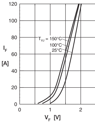
Fig. 1 Forward current vs. voltage drop
