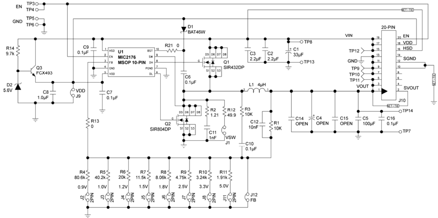
Figure 7. Schematic of MIC2176 Evaluation Board
