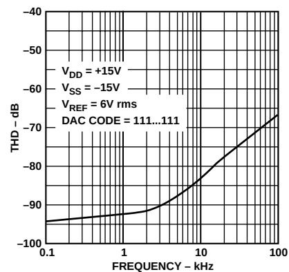
Figure 6. THD vs. Frequency
