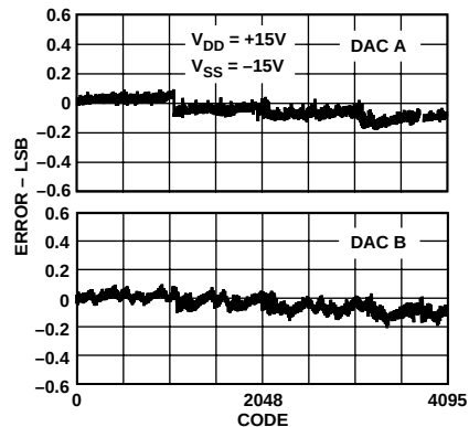
Figure 3. DAC-to-DAC Linearity Matching
