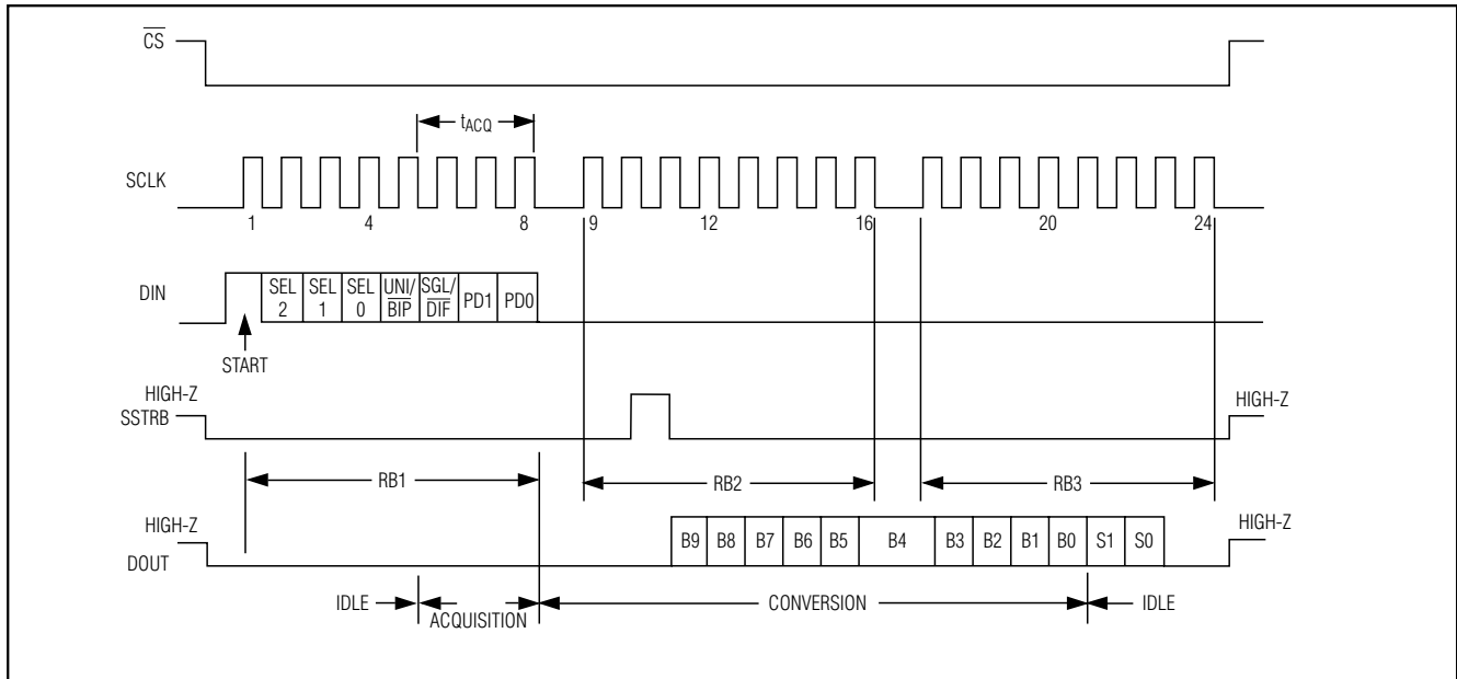
Figure 6. Single-Conversion Timing
