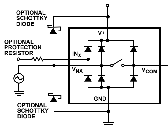
FIGURE 8. OVERVOLTAGE PROTECTION
