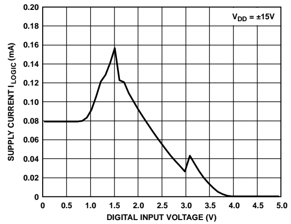
Figure 16. Supply Current I_{LOGIC} vs. Digital Input Voltage
