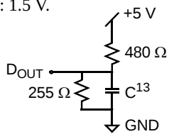
Figure B: 5 V Output load
